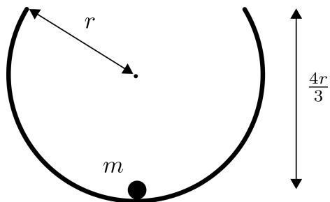
Figure 2.4: A marble at rest at the bottom of a fishbowl.
