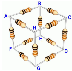
Figure 2.7: A network of 12 identical resistors of resistance R
