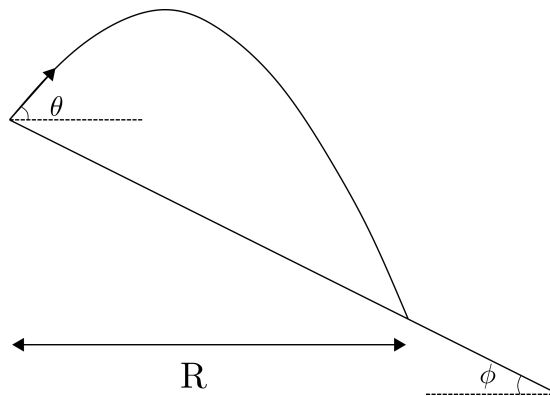
Figure 2.6: The trajectory of a cannonball being fired at an angle \theta to the horizontal at the top of a hill with an incline of \phi .
