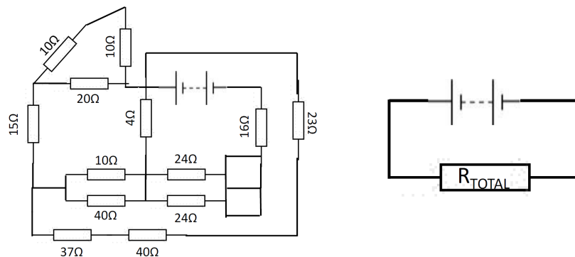
Figure 2.3: Two resistor networks
